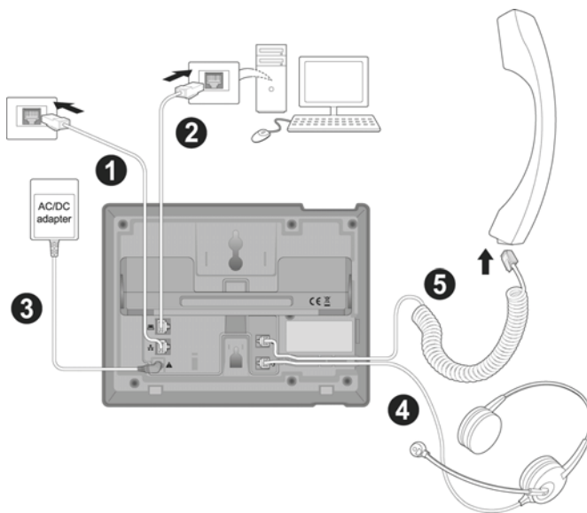
Figure 2: IP Phone Connections
